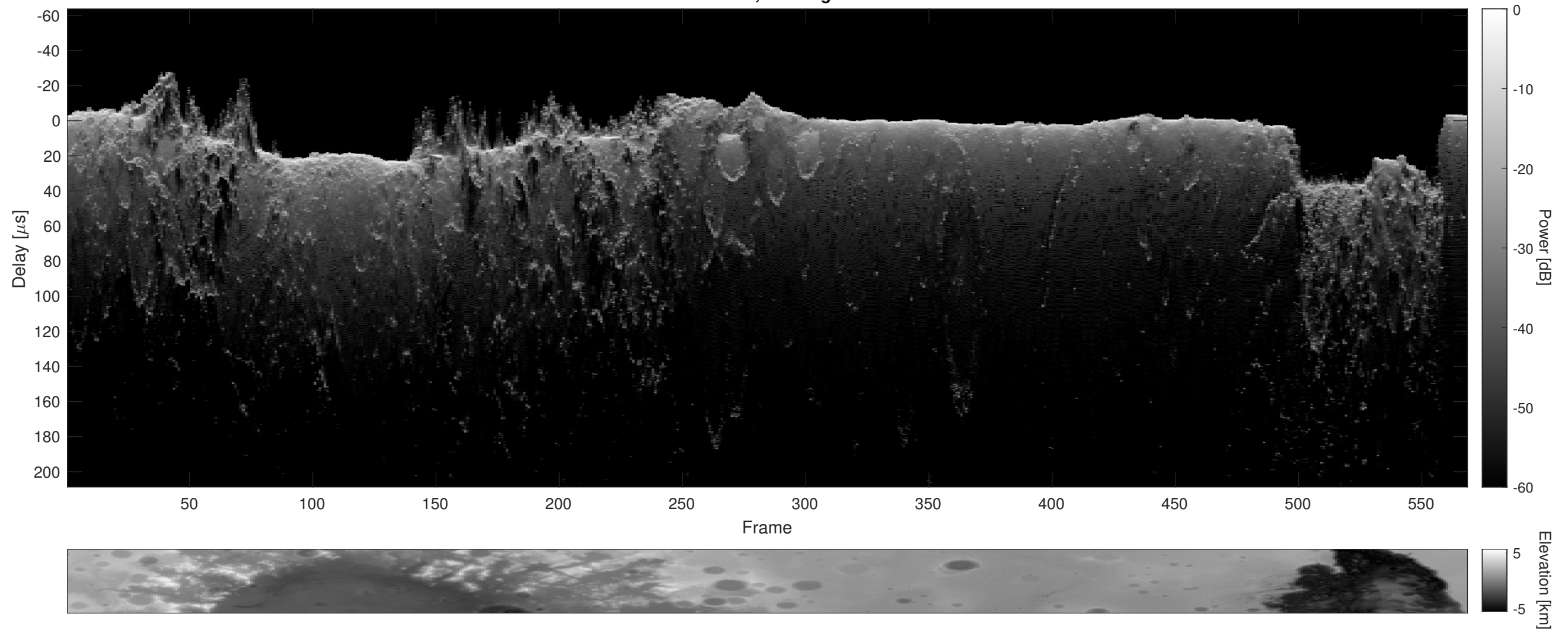
Orbit 6194, Cluttergram
