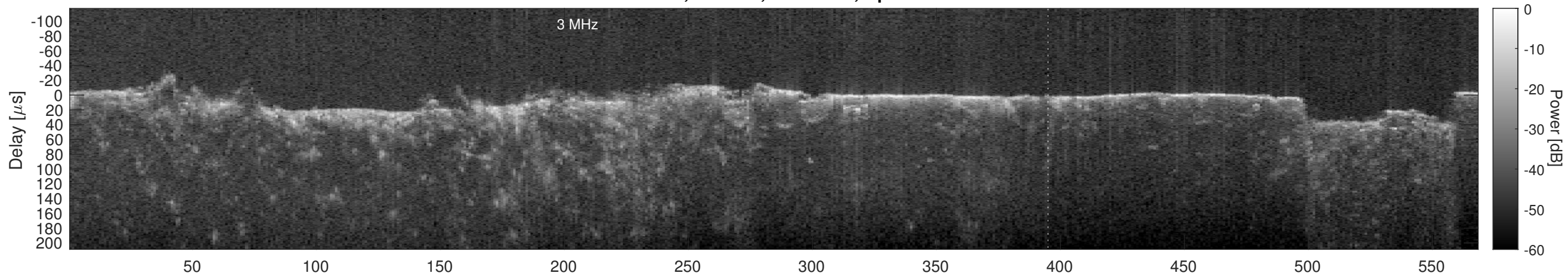
Orbit 6194, Cluttergram
