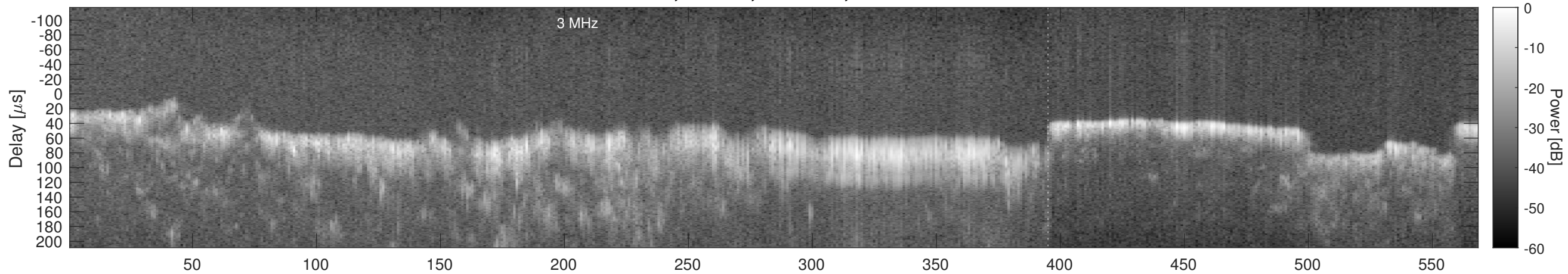
Orbit 6194, Window, Channel 2, Chapman
