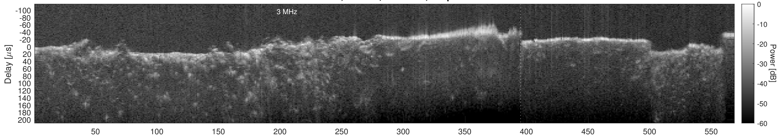
Orbit 6194, Window, Channel 2, Optimized
