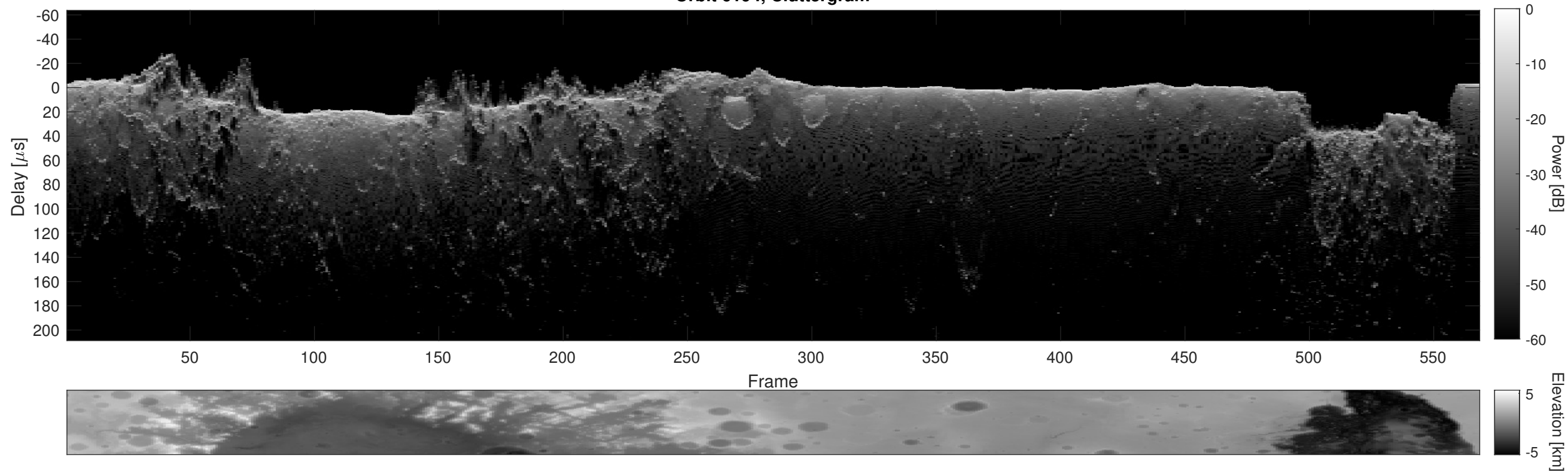
Orbit 6194, Cluttergram
