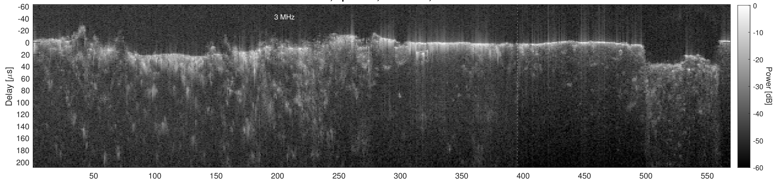
Orbit 6194, Cluttergram
