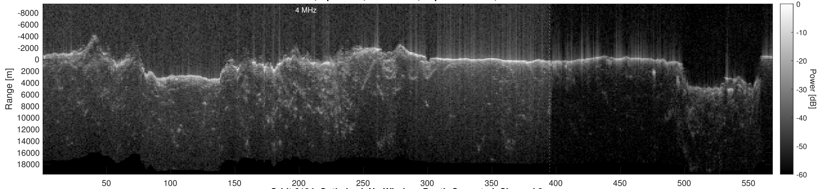
Orbit 6194, Optimized, No Window, Depth-Corrected, Channel 2
