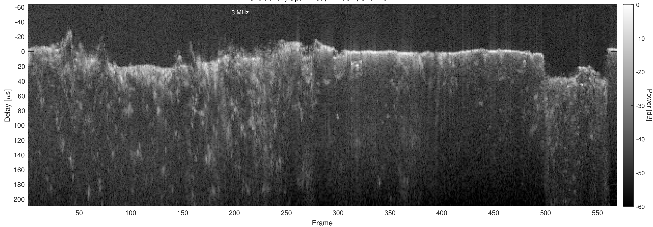
Orbit 6194, Optimized, Window, Channel 2
