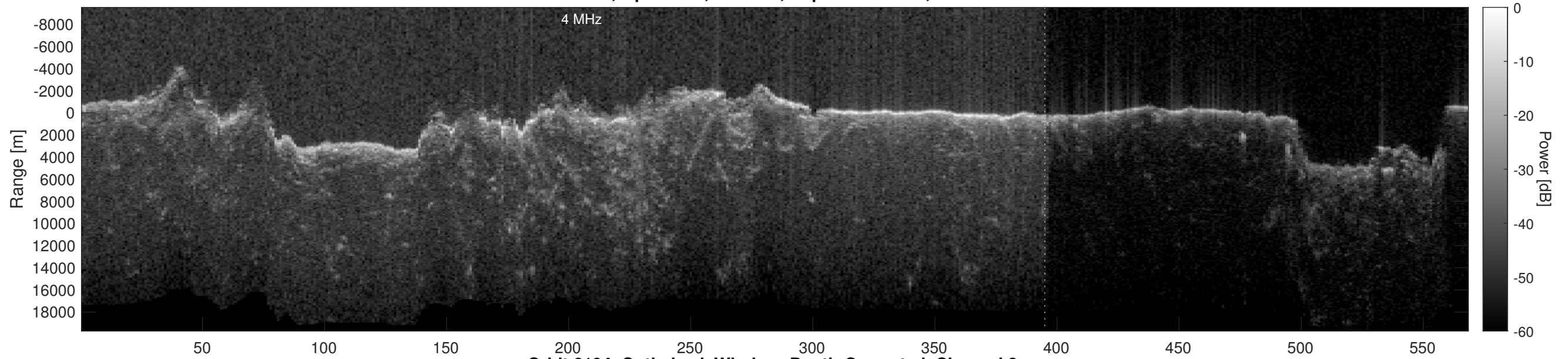
Orbit 6194, Optimized, Window, Depth-Corrected, Channel 2
