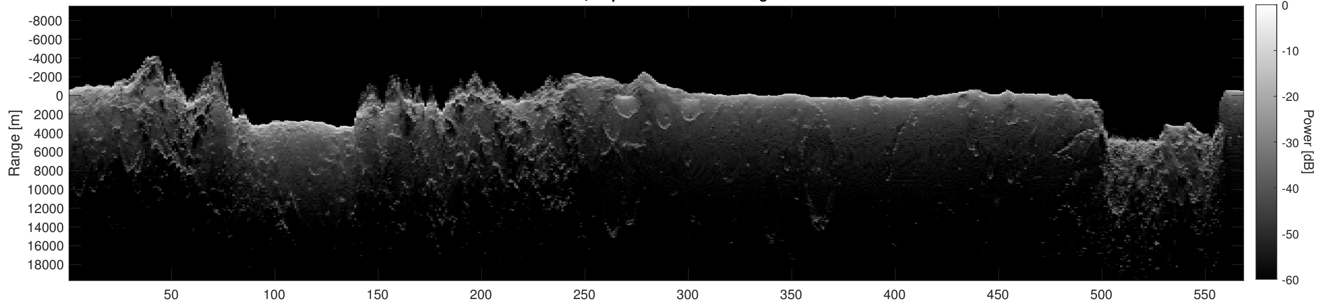
Orbit 6194, Depth-Corrected Cluttergram
