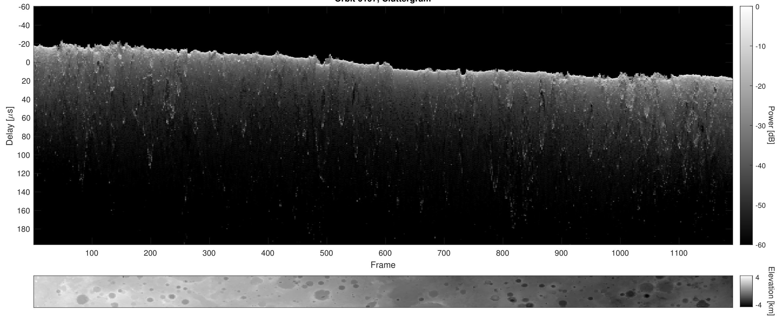
Orbit 6197, Cluttergram
