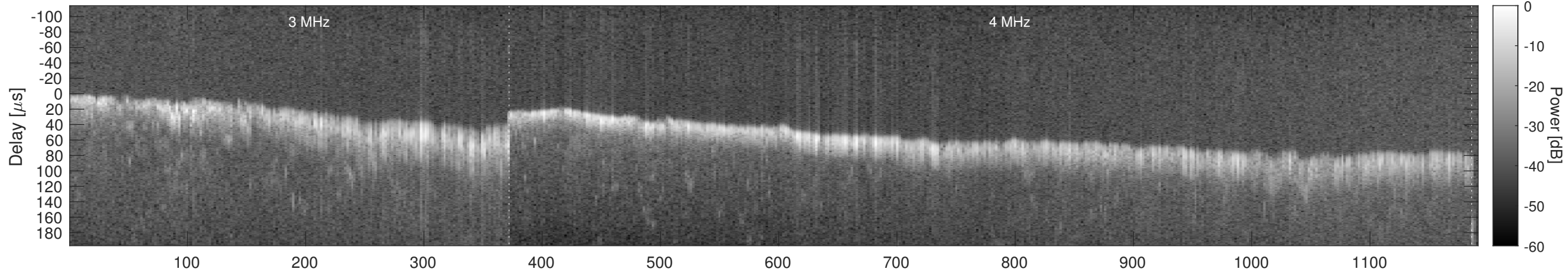
Orbit 6197, Window, Channel 2, Chapman
