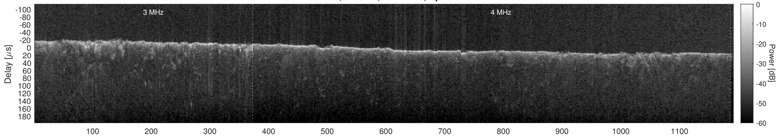
Orbit 6197, Cluttergram
