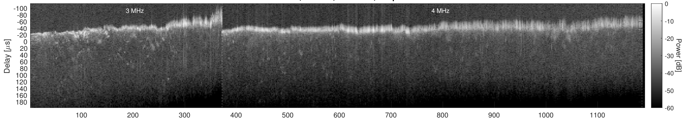
Orbit 6197, Window, Channel 2, Optimized
