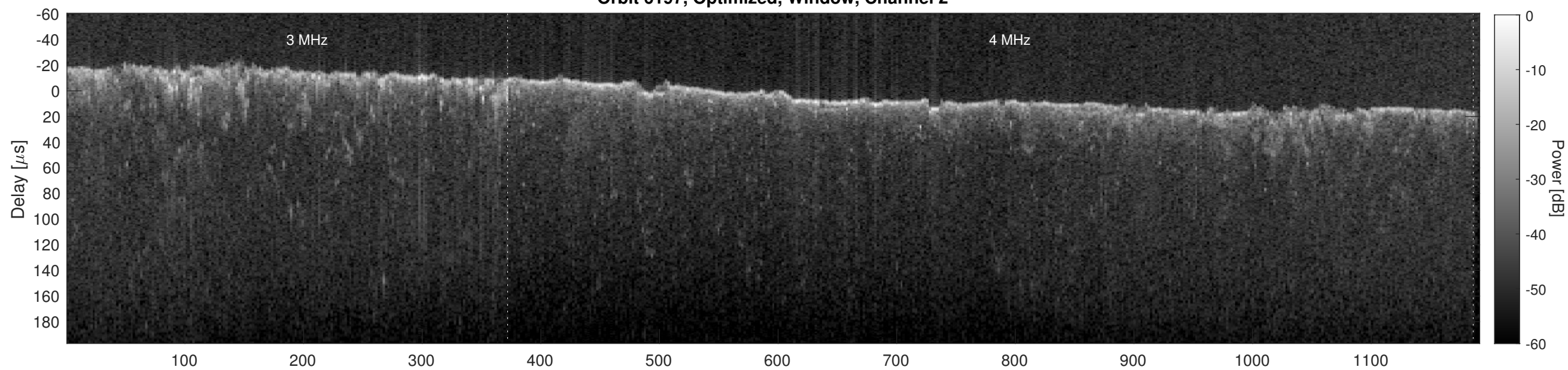
Orbit 6197, Cluttergram
