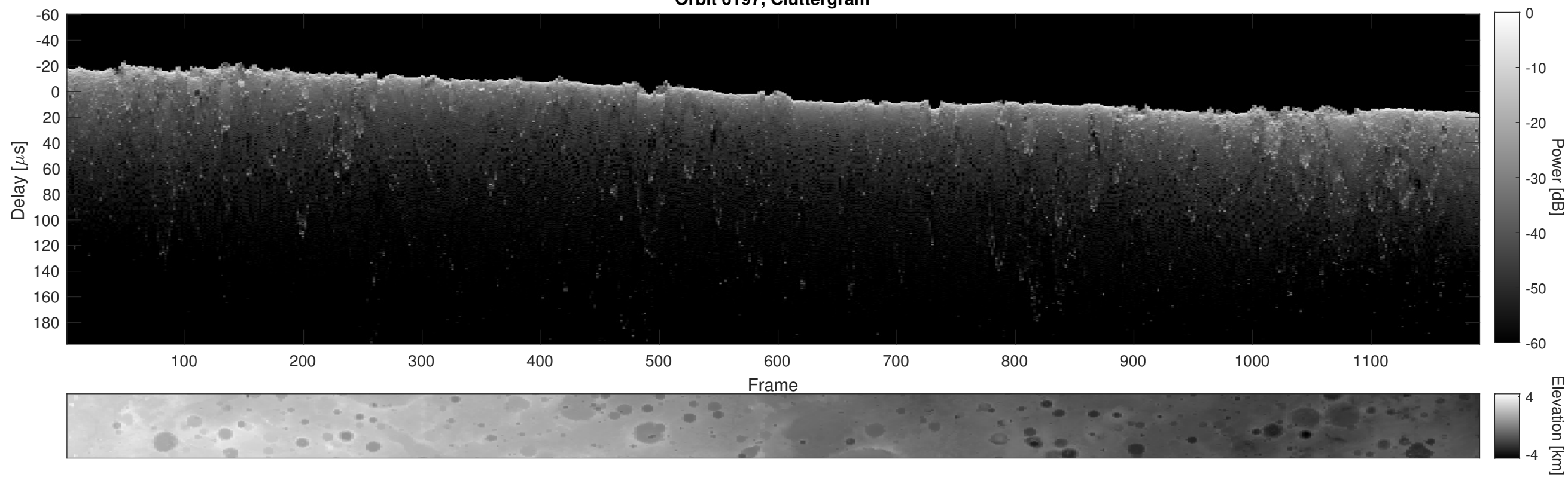
Orbit 6197, Cluttergram
