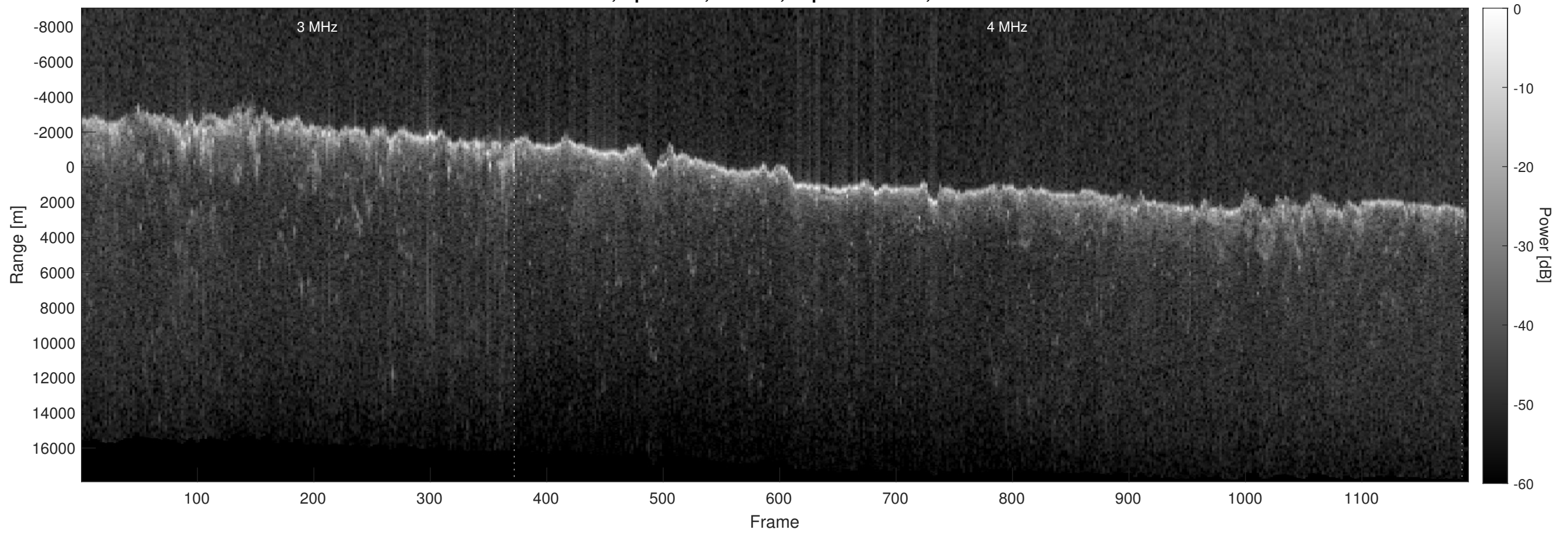
Orbit 6197, Optimized, Window, Depth-Corrected, Channel 2
