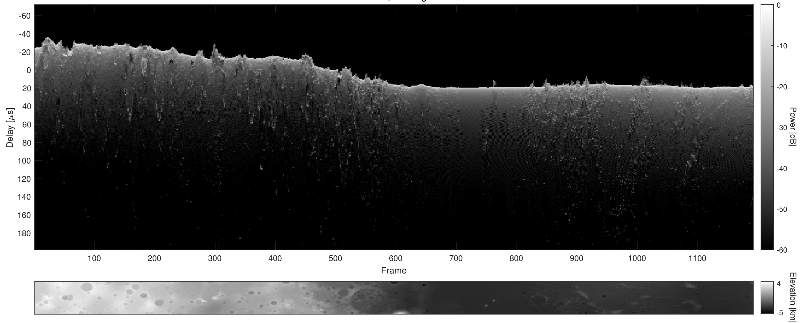
Orbit 6199, Cluttergram
