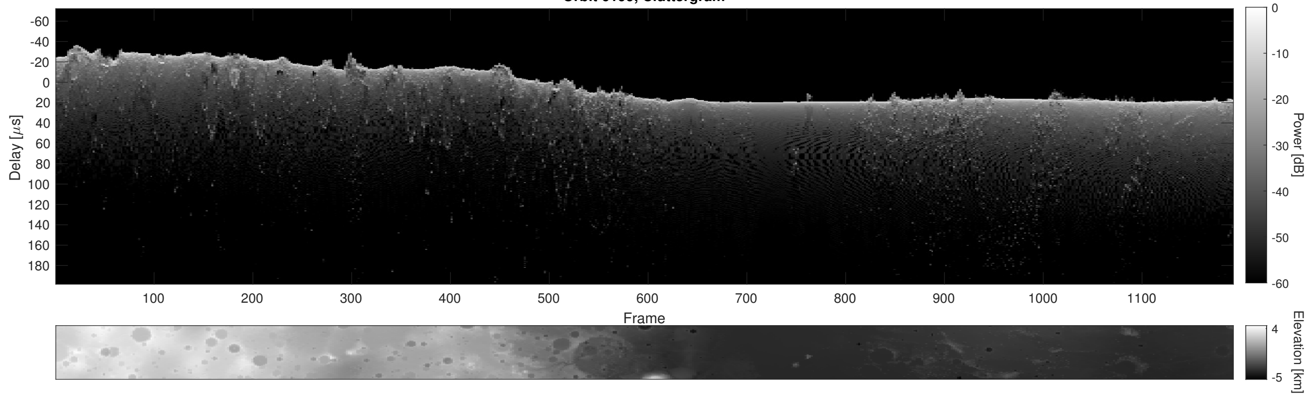
Orbit 6199, Cluttergram
