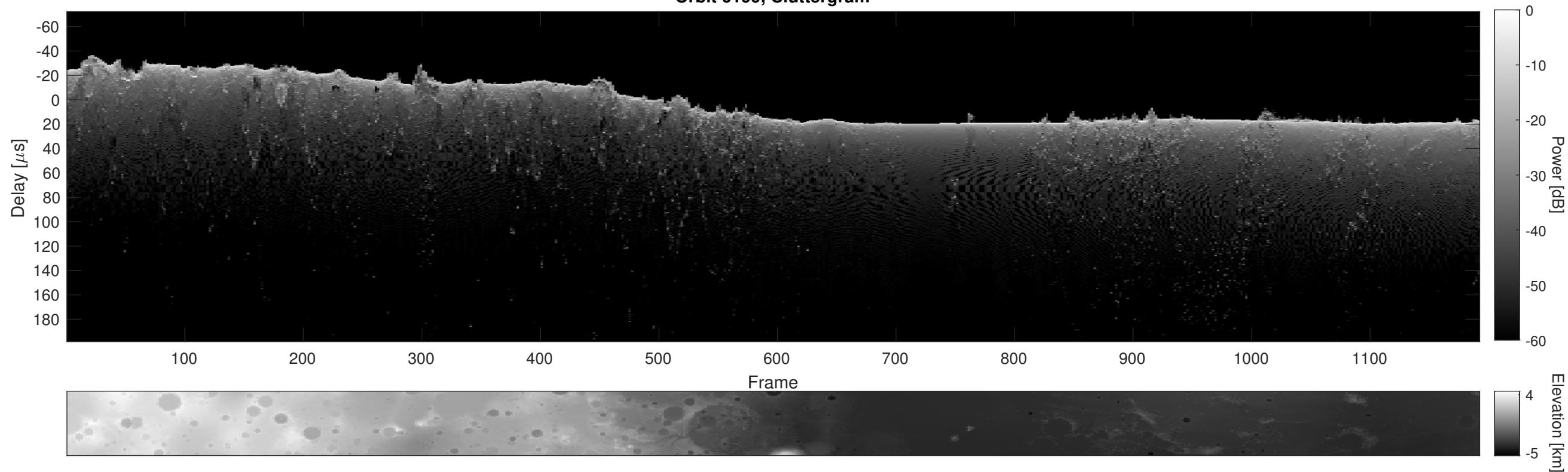
Orbit 6199, Cluttergram
