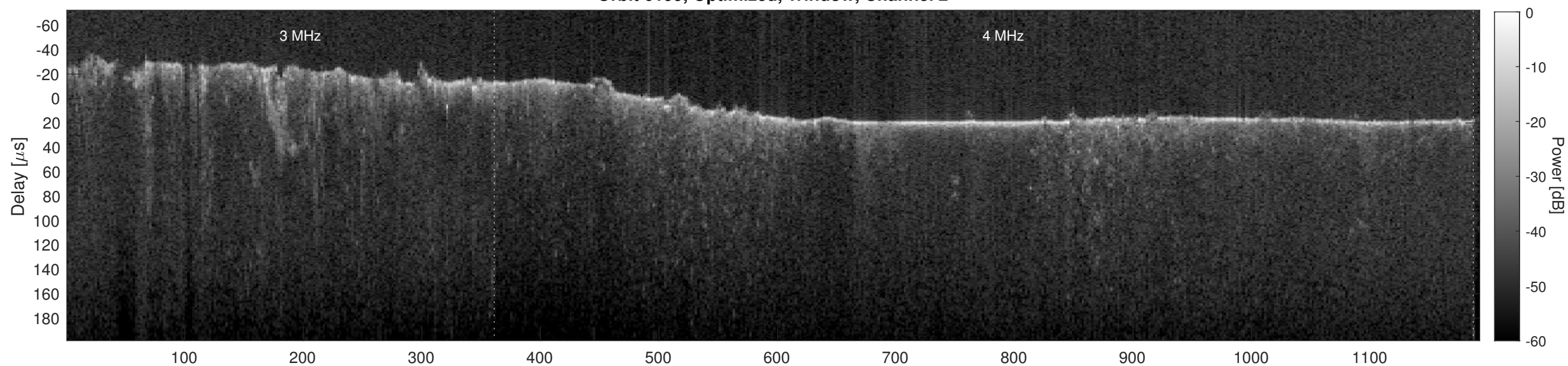
Orbit 6199, Cluttergram
