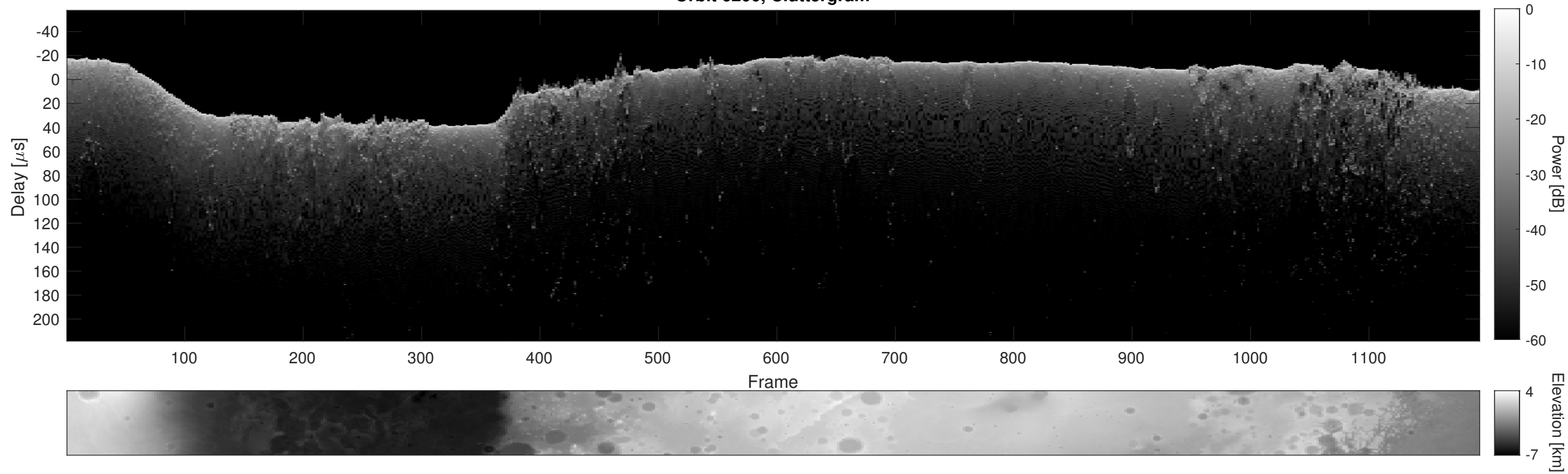
Orbit 6200, Cluttergram
