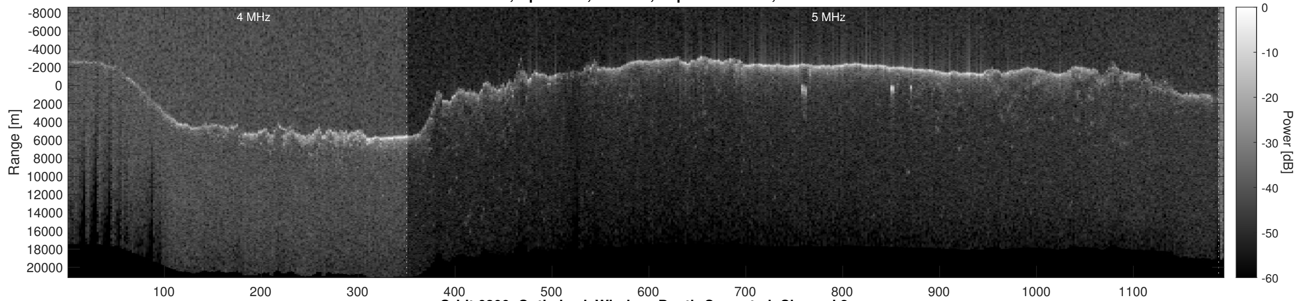
Orbit 6200, Optimized, Window, Depth-Corrected, Channel 2
