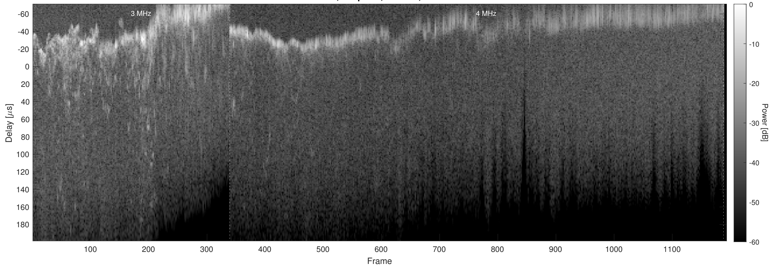
Orbit 6201, Chapman, Window, Channel 2
