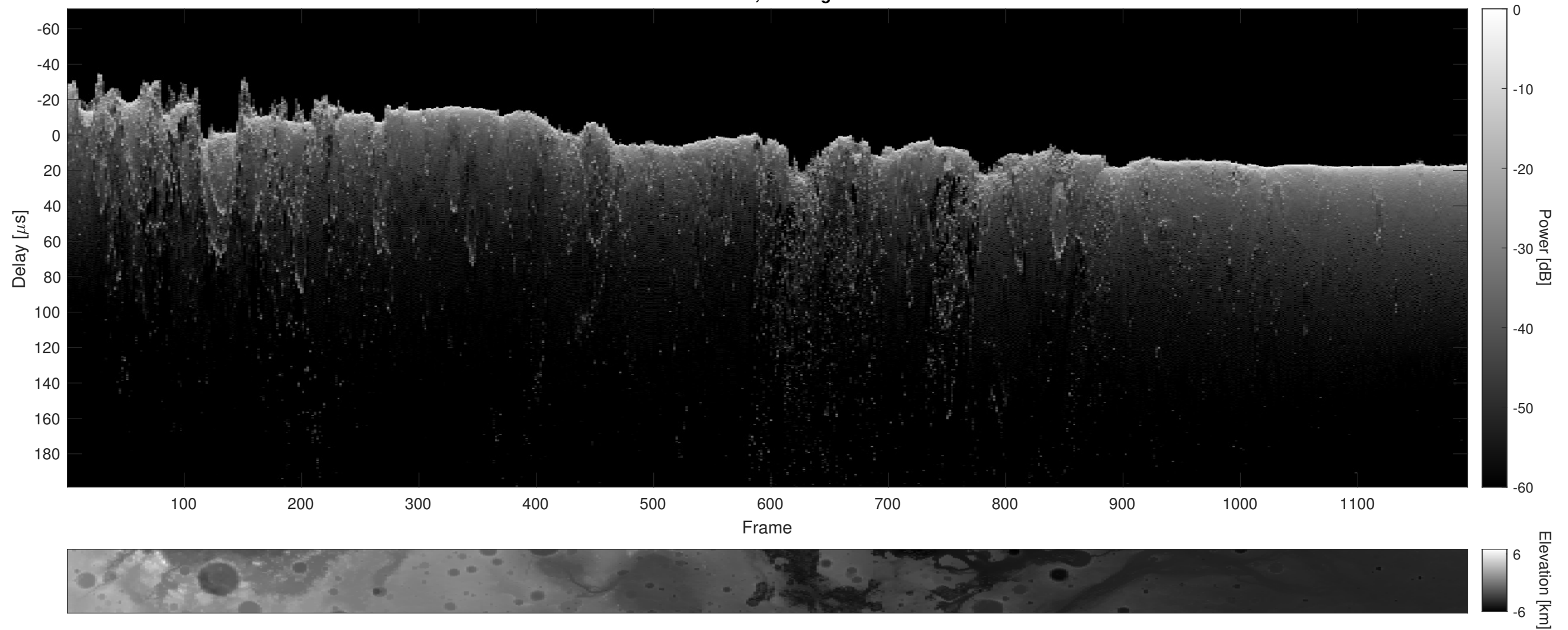
Orbit 6201, Cluttergram
