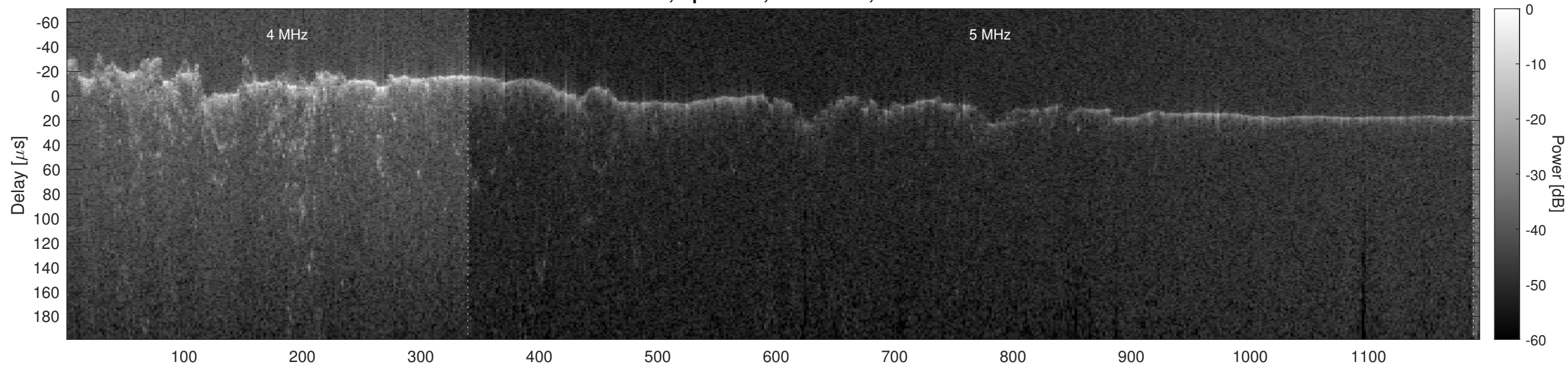
Orbit 6201, Optimized, No Window, Channel 2
