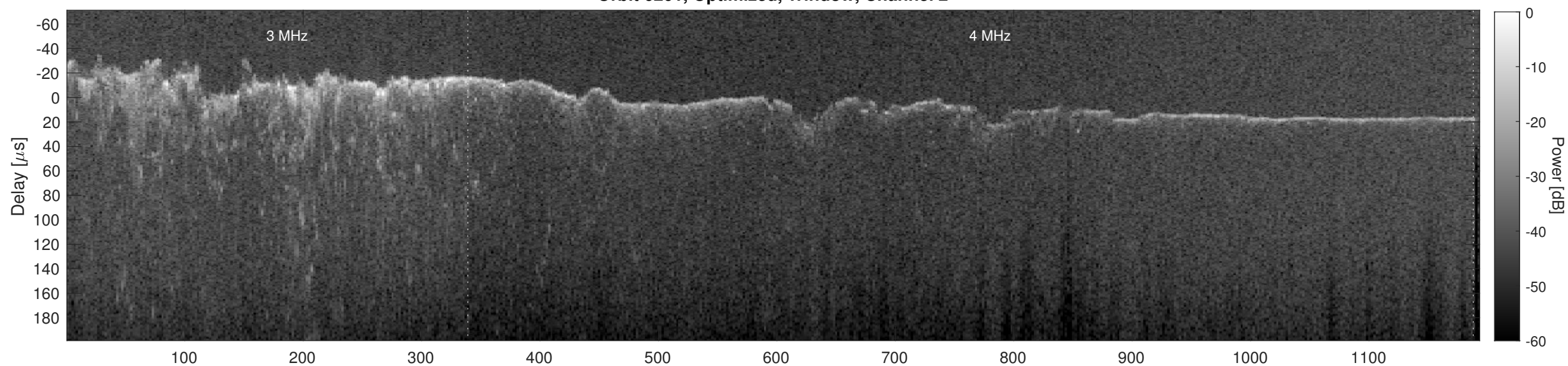
Orbit 6201, Cluttergram
