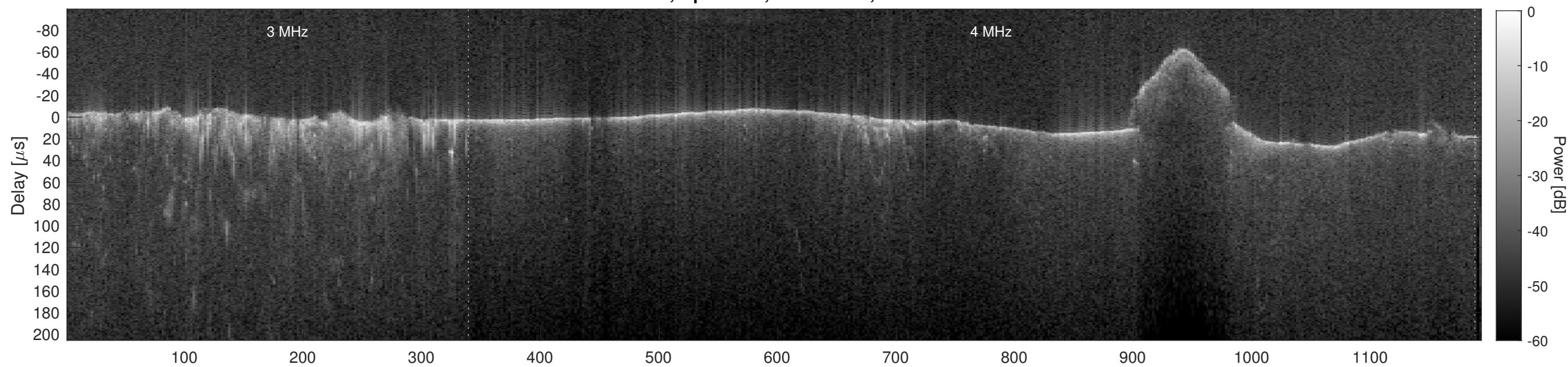
Orbit 6202, Cluttergram
