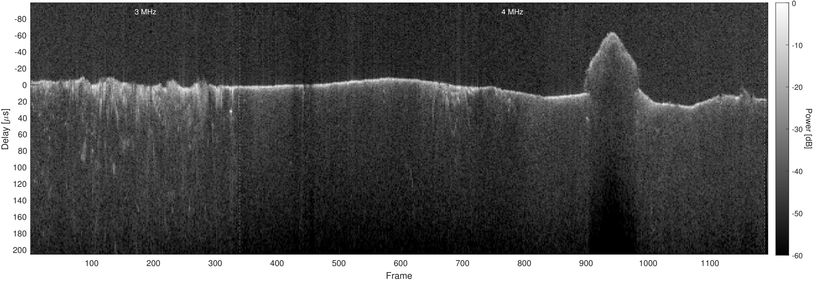
Orbit 6202, Optimized, Window, Channel 2
