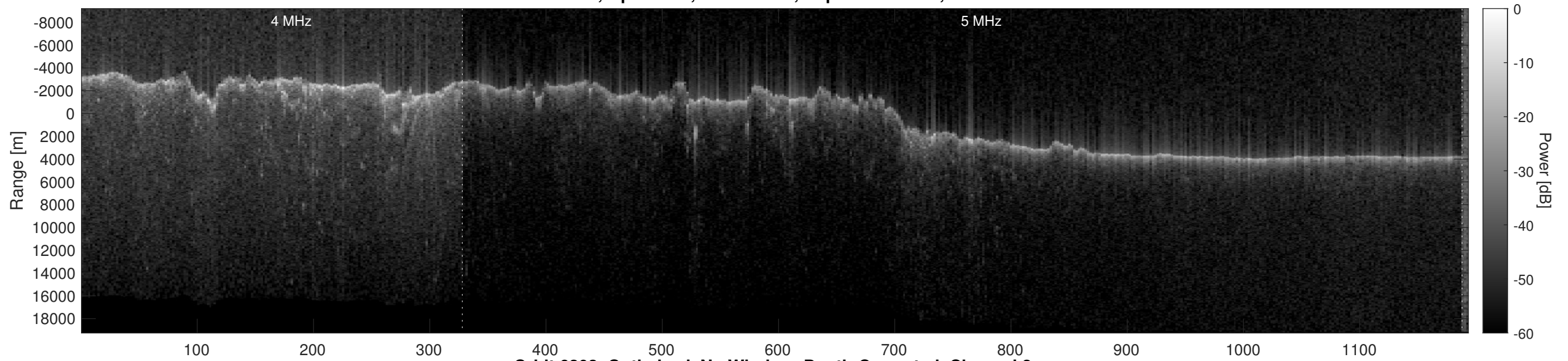
Orbit 6203, Optimized, No Window, Depth-Corrected, Channel 2
