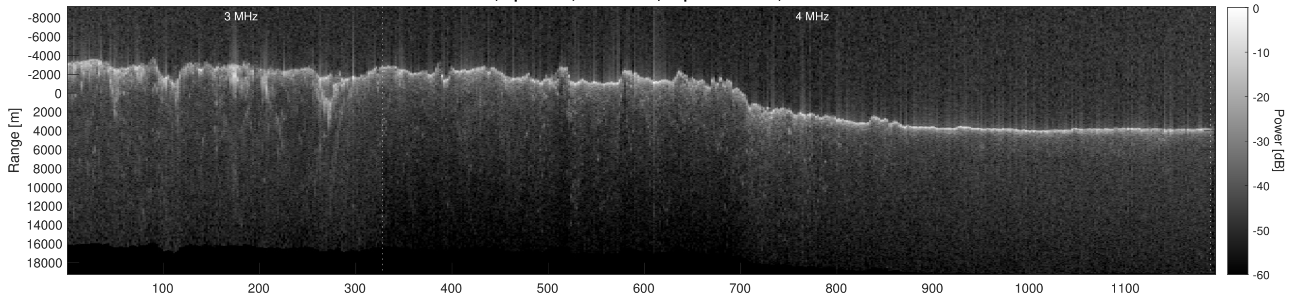
Orbit 6203, Depth-Corrected Cluttergram
