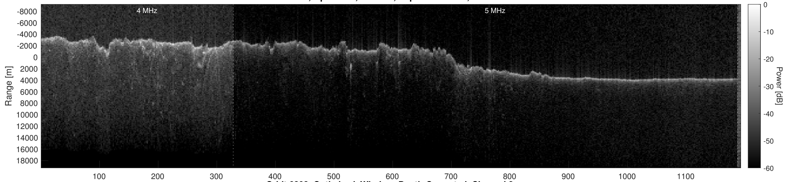
Orbit 6203, Optimized, Window, Depth-Corrected, Channel 2
