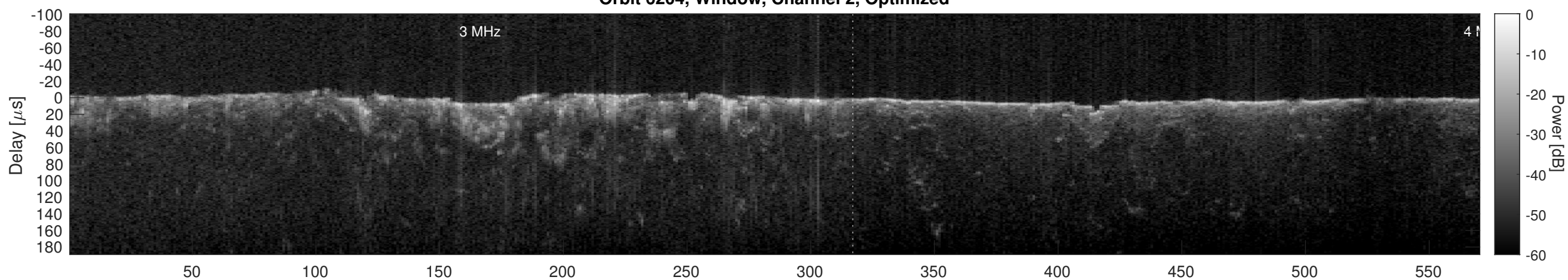
Orbit 6204, Cluttergram
