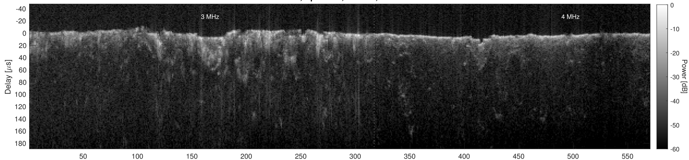
Orbit 6204, Cluttergram
