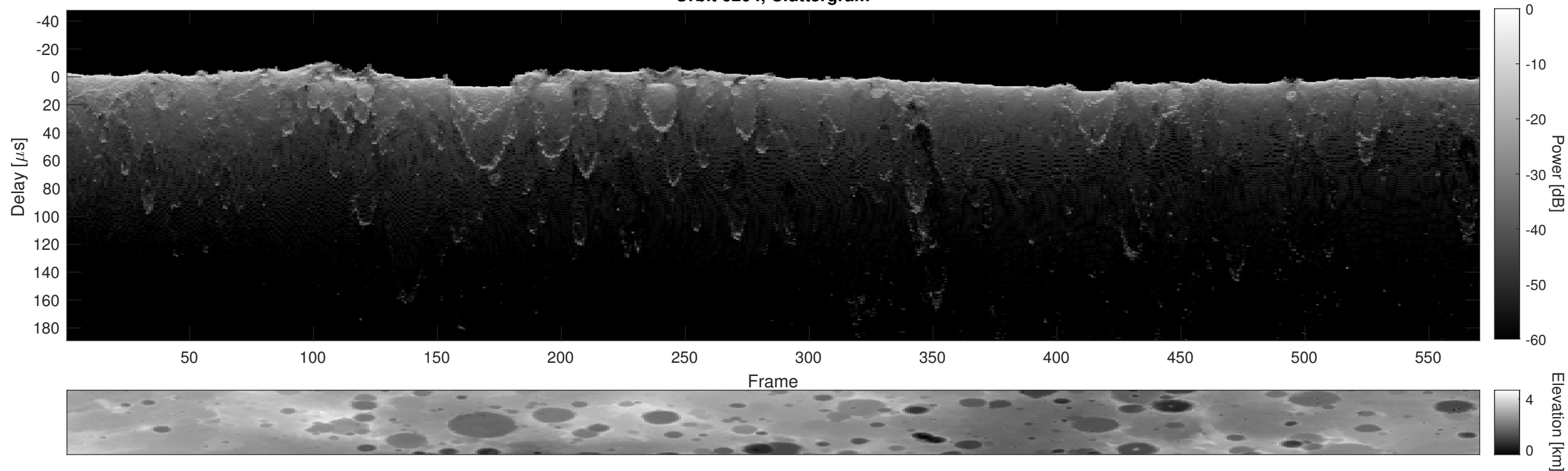
Orbit 6204, Cluttergram
