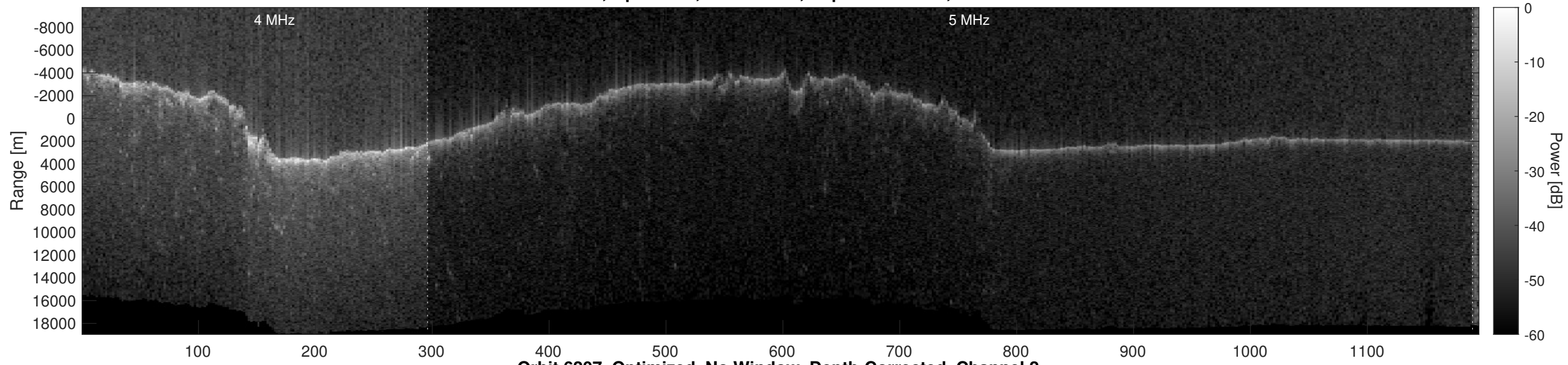
Orbit 6207, Optimized, No Window, Depth-Corrected, Channel 2
