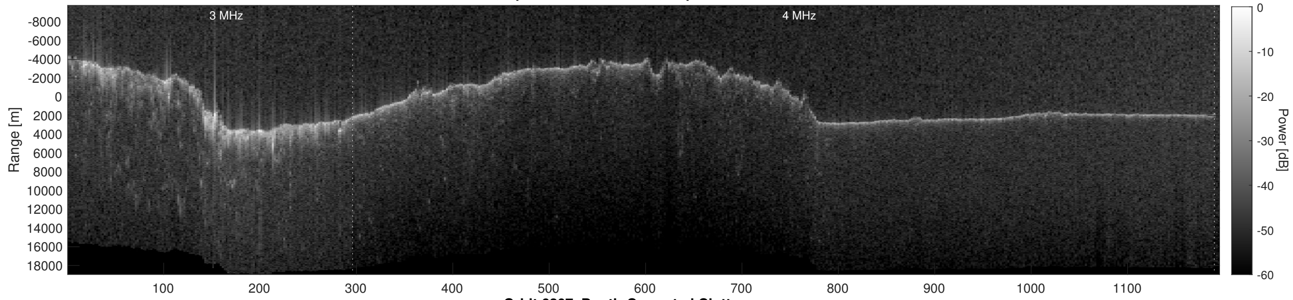
Orbit 6207, Depth-Corrected Cluttergram
