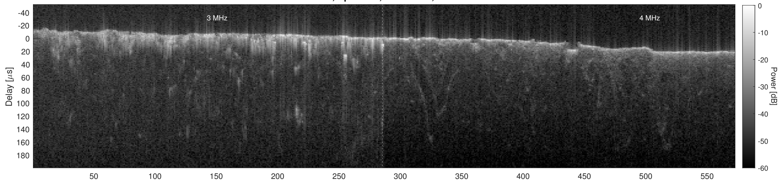
Orbit 6208, Cluttergram
