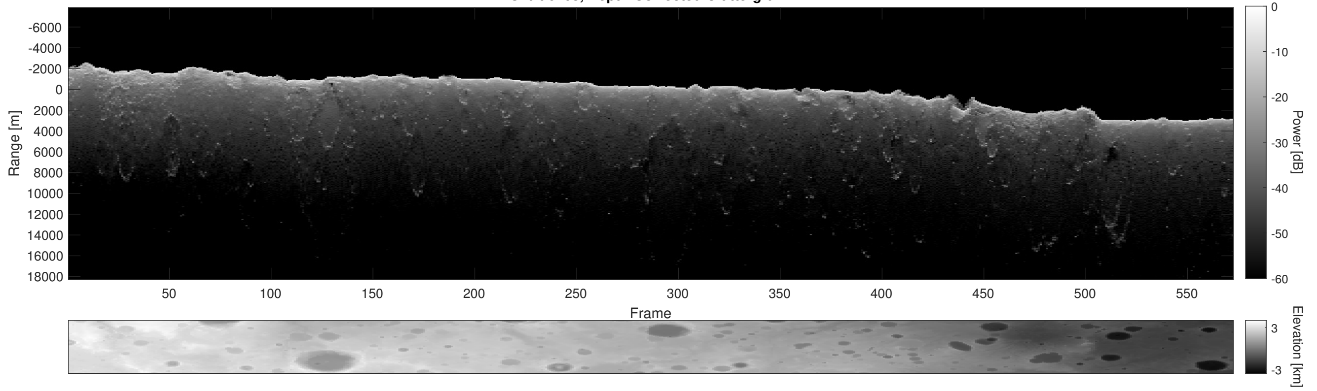
Orbit 6208, Depth-Corrected Cluttergram
