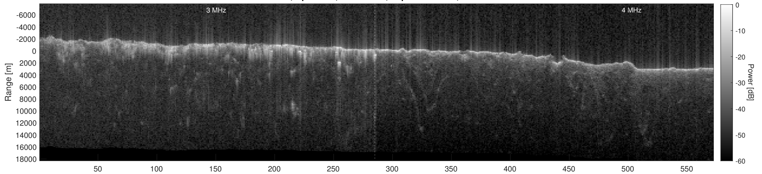
Orbit 6208, Depth-Corrected Cluttergram
