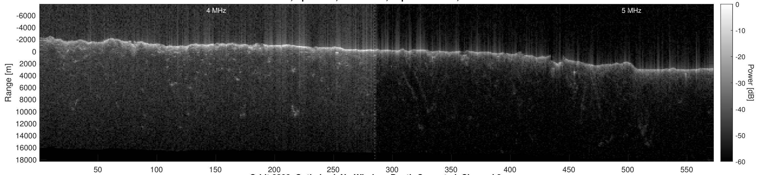
Orbit 6208, Optimized, No Window, Depth-Corrected, Channel 2
