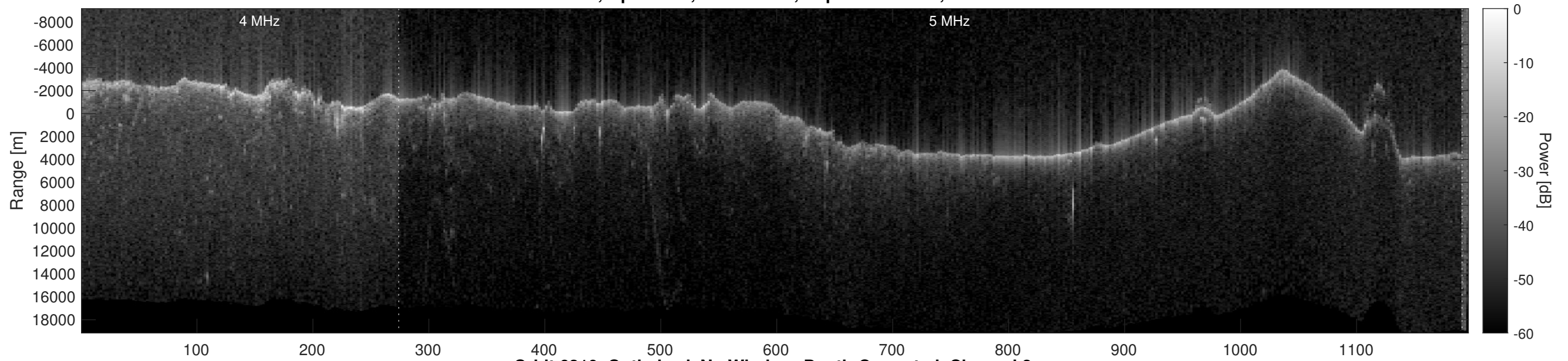
Orbit 6210, Optimized, No Window, Depth-Corrected, Channel 2
