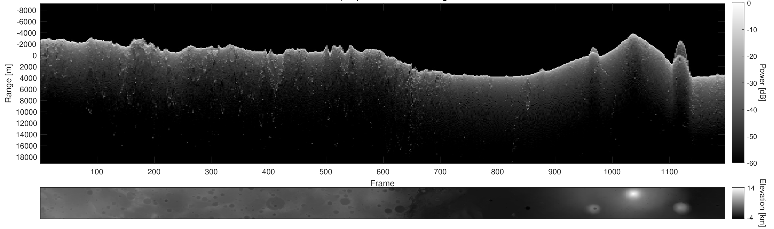
Orbit 6210, Depth-Corrected Cluttergram
