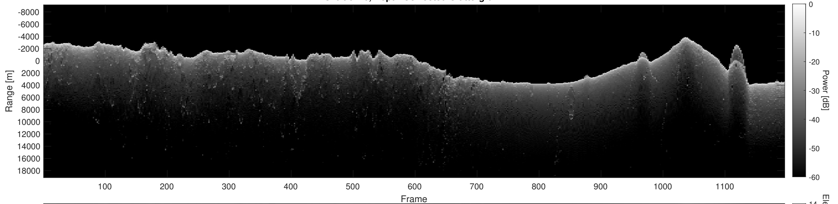
Orbit 6210, Depth-Corrected Cluttergram
