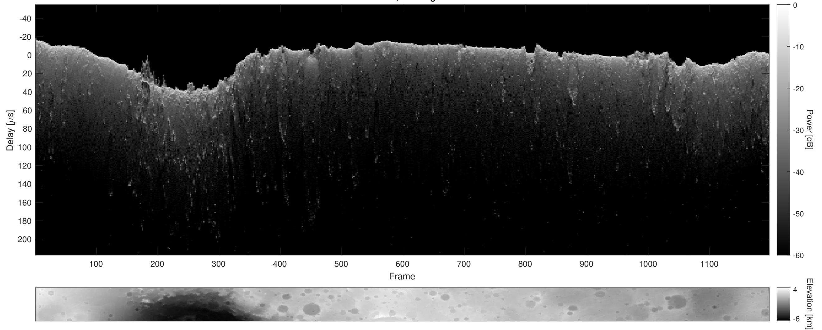
Orbit 6211, Cluttergram
