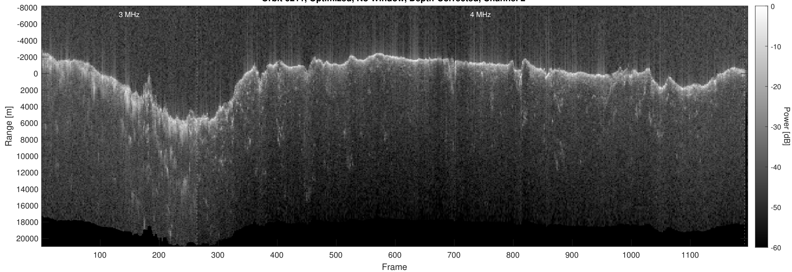
Orbit 6211, Optimized, No Window, Depth-Corrected, Channel 2
