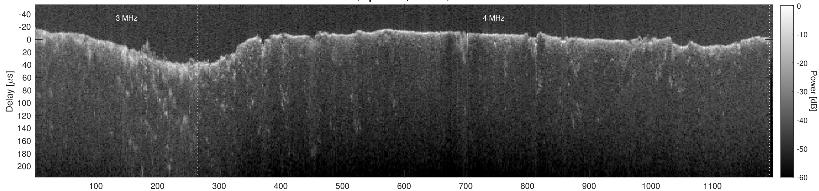
Orbit 6211, Cluttergram
