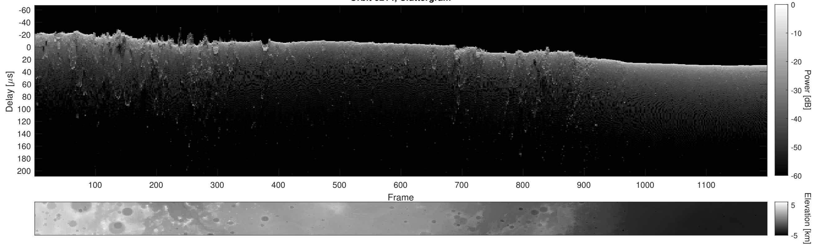
Orbit 6214, Cluttergram
