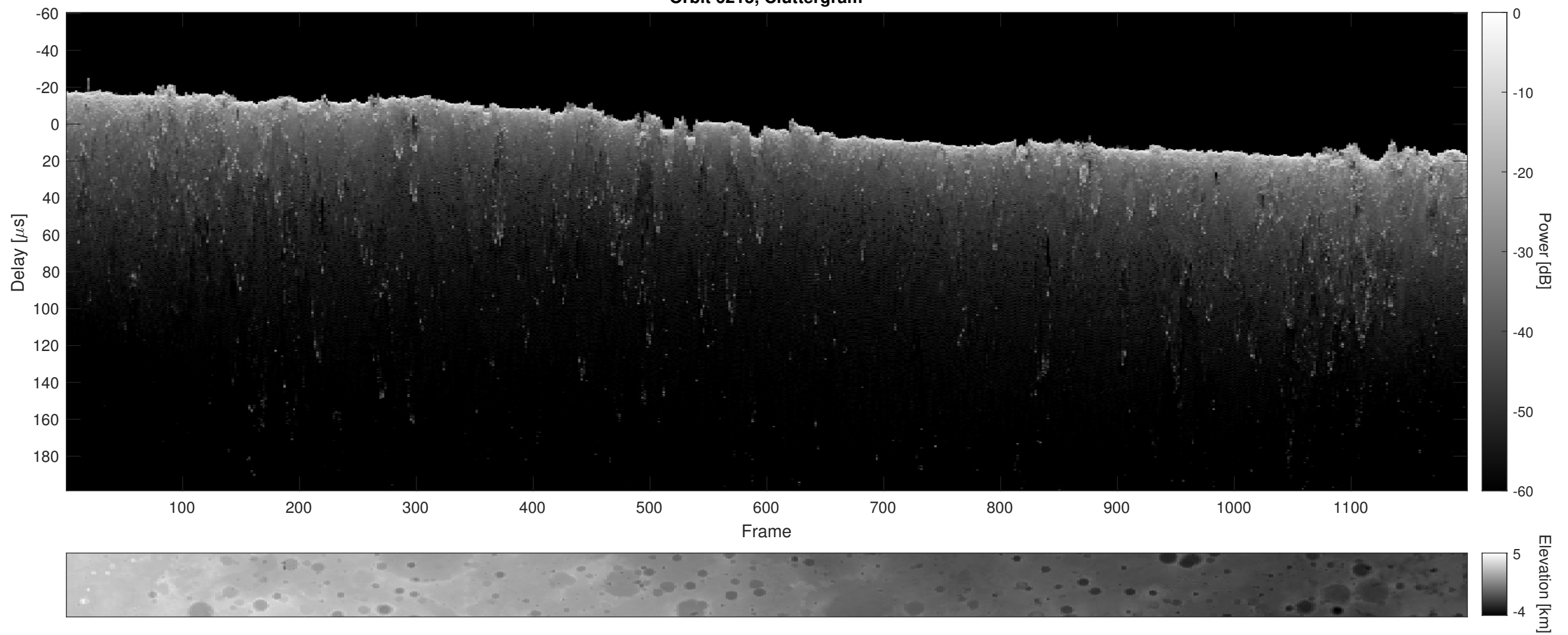
Orbit 6215, Cluttergram
