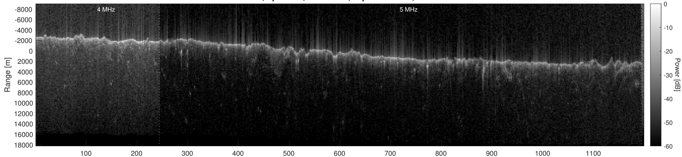
Orbit 6215, Optimized, No Window, Depth-Corrected, Channel 2
