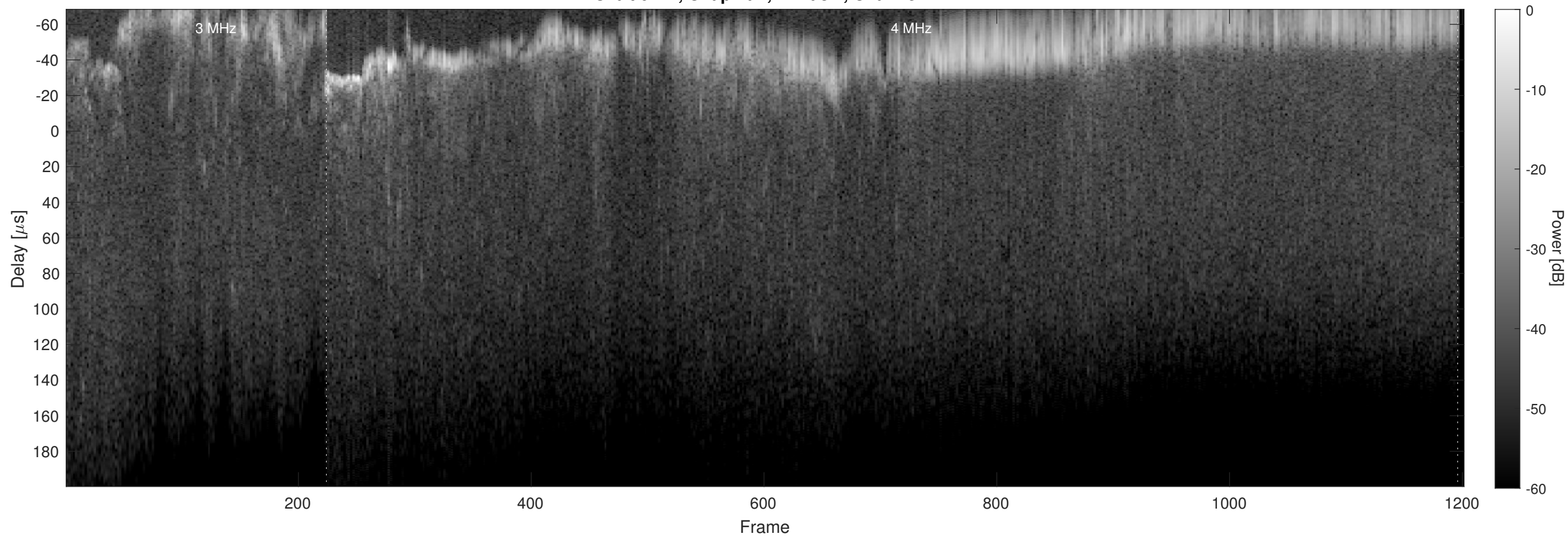
Orbit 6217, Chapman, Window, Channel 2
