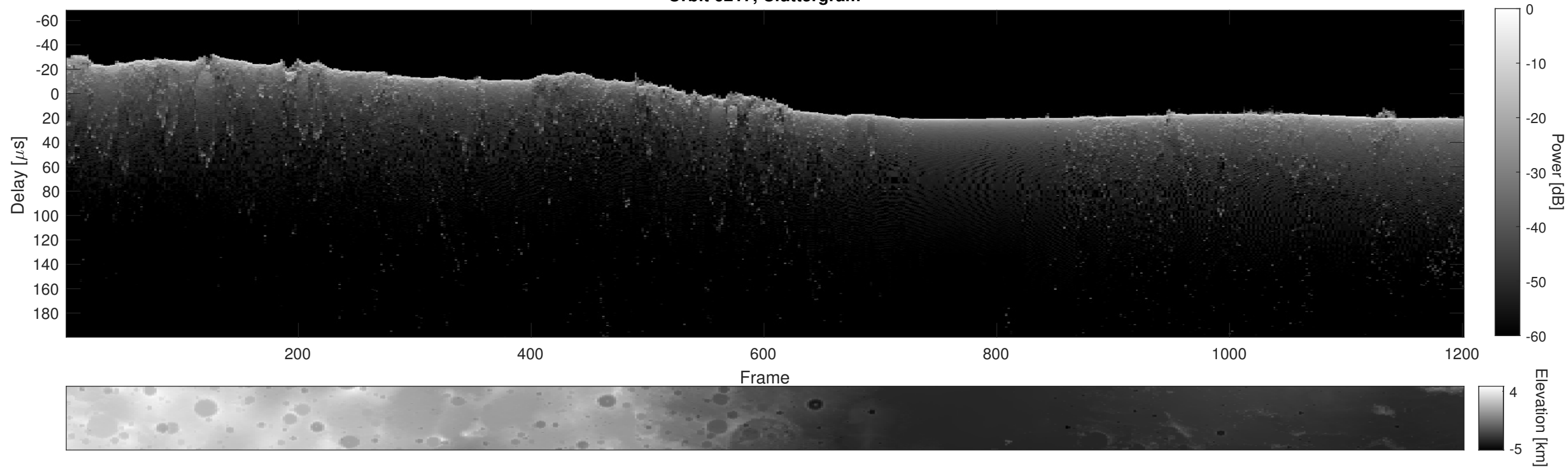
Orbit 6217, Cluttergram
