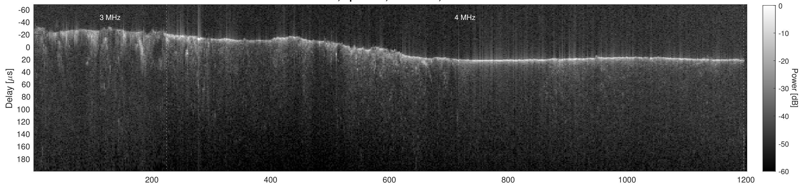
Orbit 6217, Cluttergram
