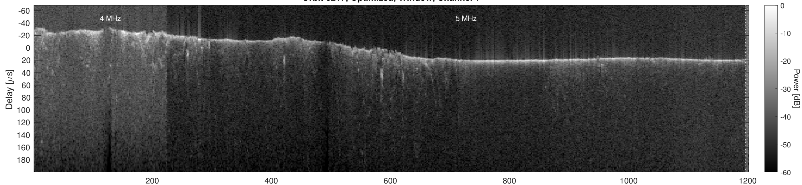
Orbit 6217, Optimized, Window, Channel 2
