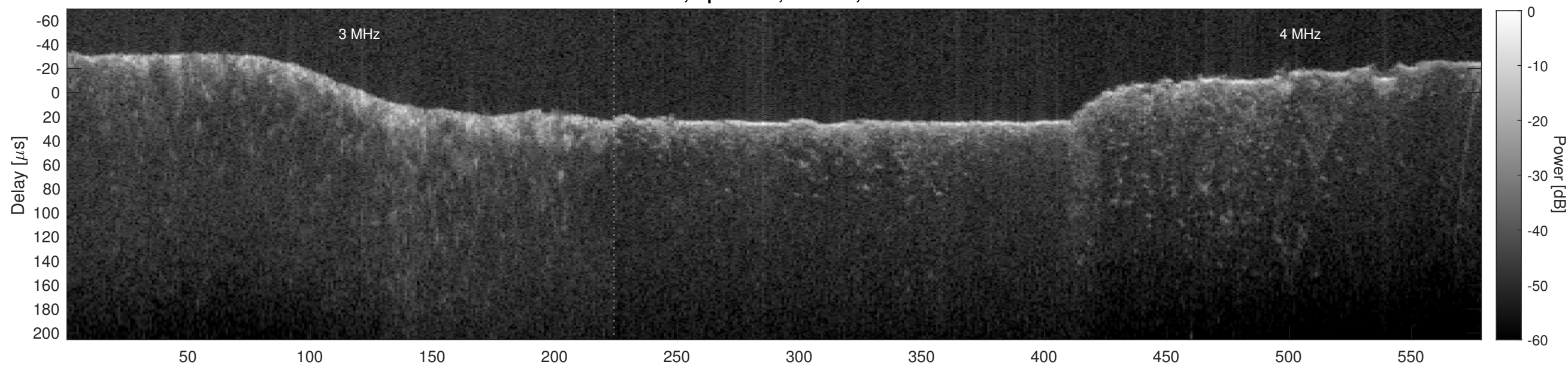
Orbit 6218, Cluttergram
