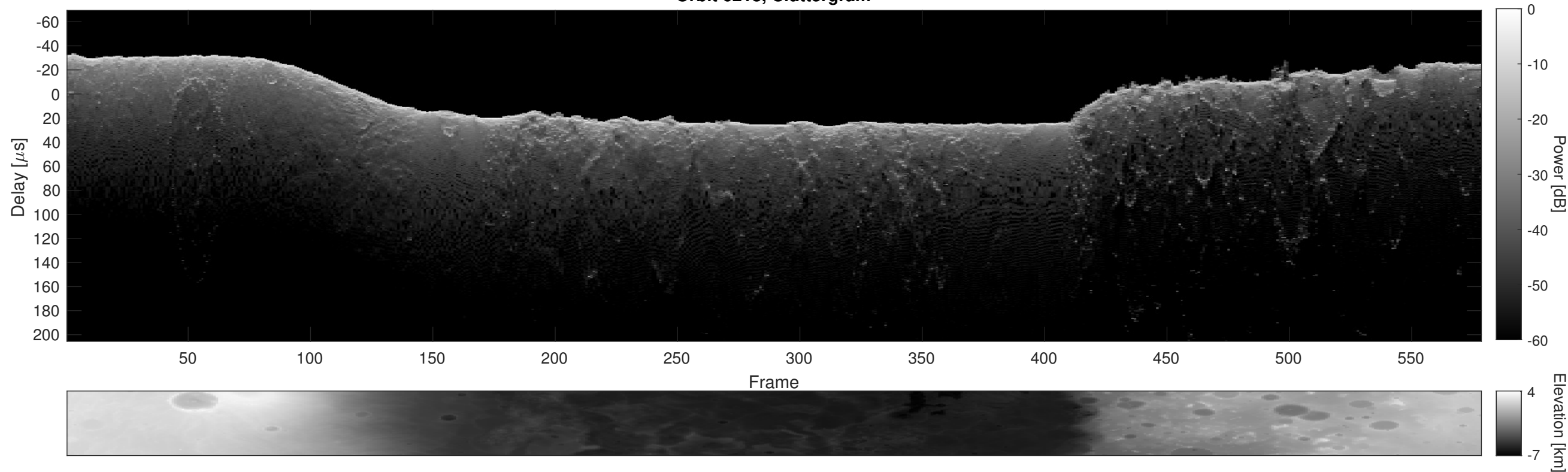
Orbit 6218, Cluttergram
