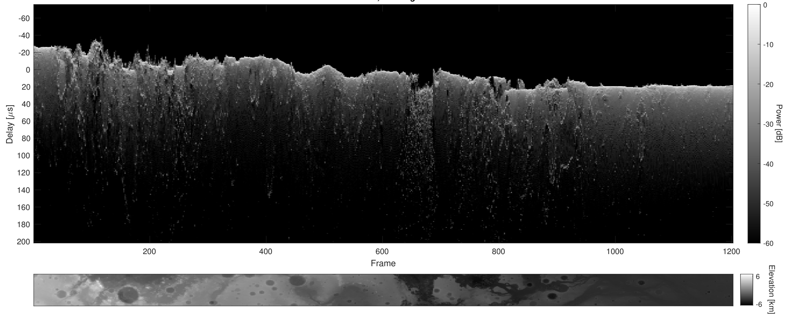
Orbit 6219, Cluttergram
