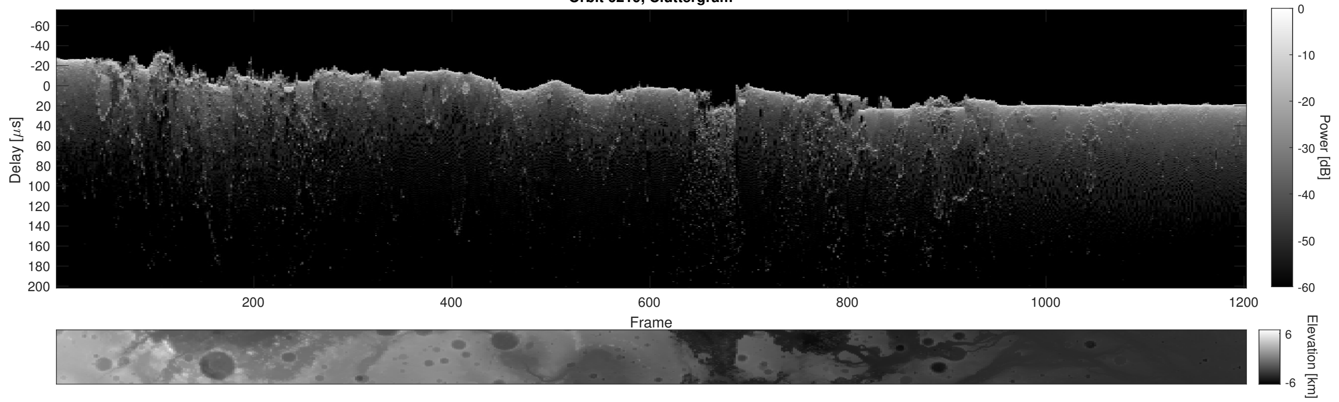
Orbit 6219, Cluttergram
