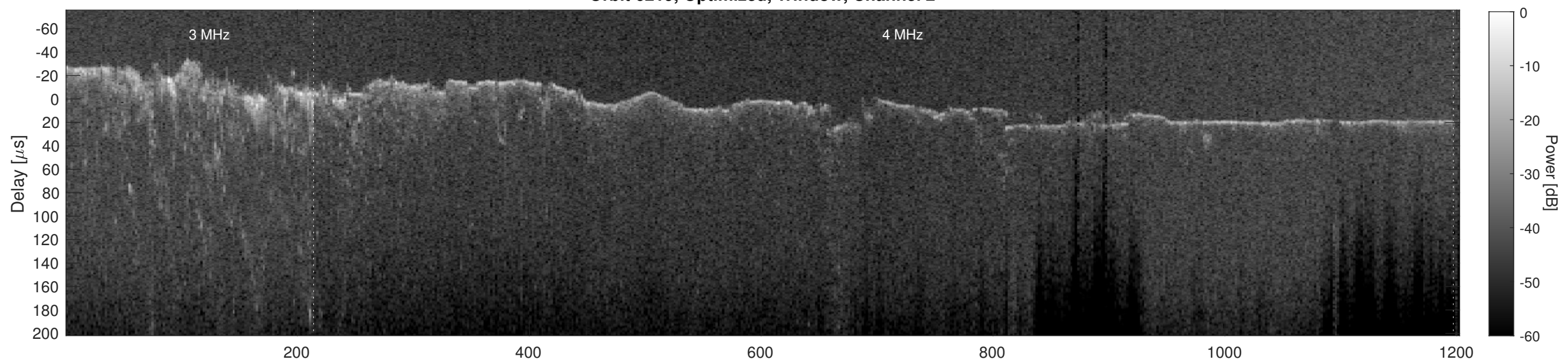
Orbit 6219, Cluttergram
