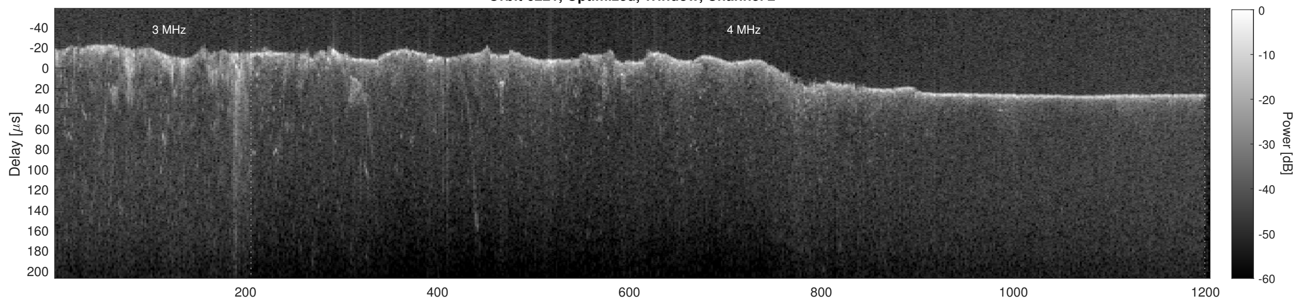
Orbit 6221, Cluttergram
