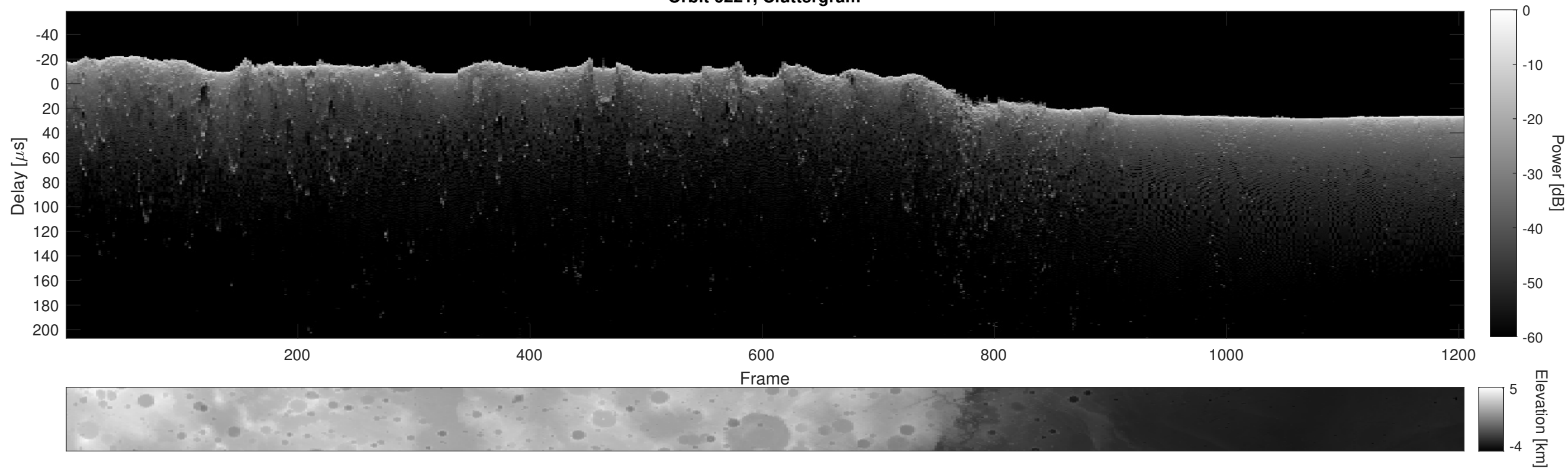
Orbit 6221, Cluttergram
