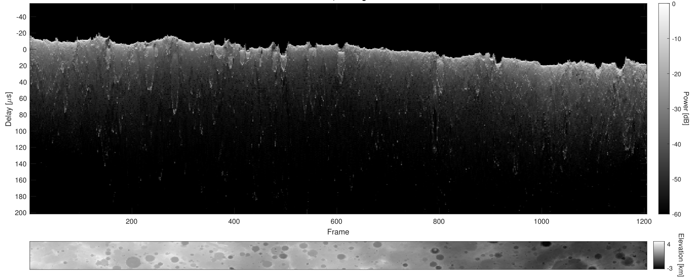
Orbit 6222, Cluttergram
