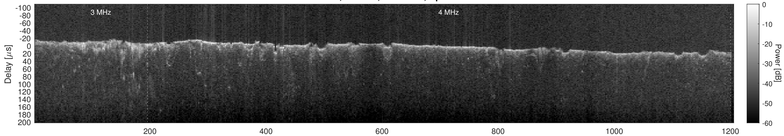
Orbit 6222, Cluttergram
