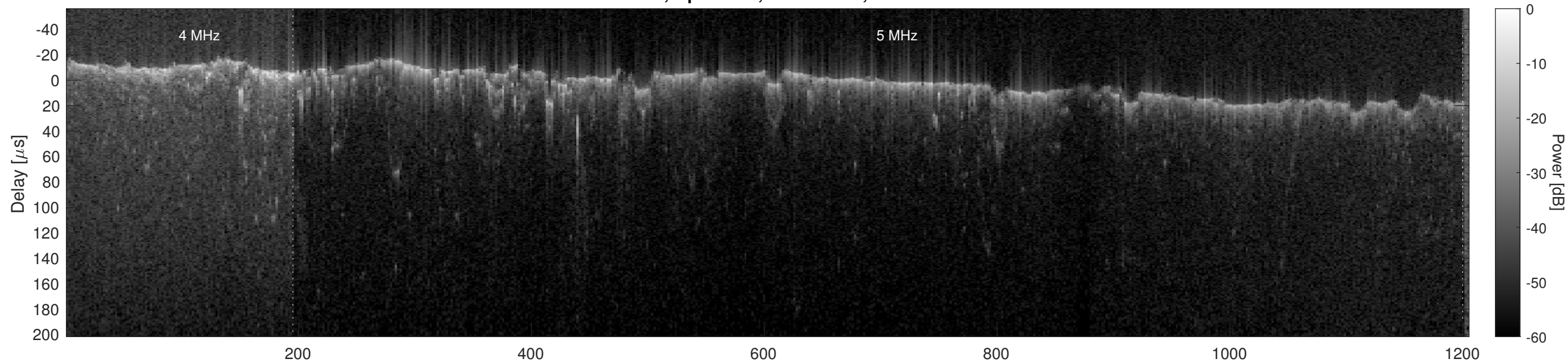
Orbit 6222, Optimized, No Window, Channel 2
