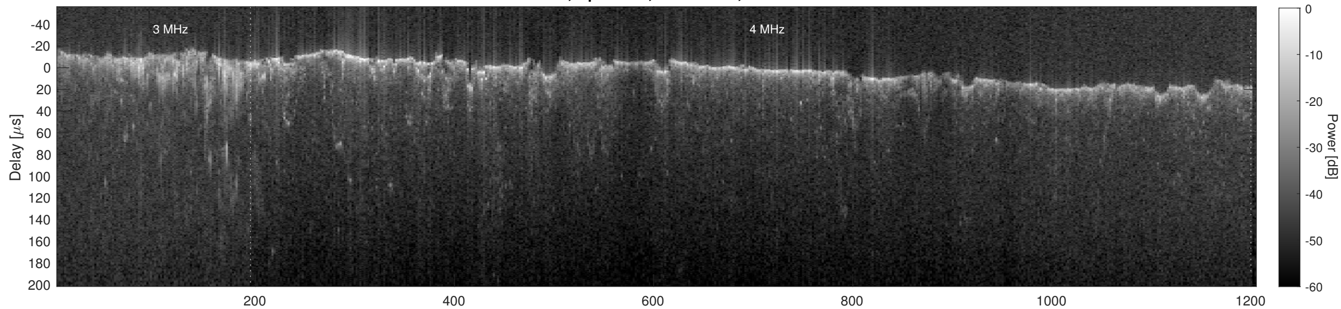
Orbit 6222, Cluttergram
