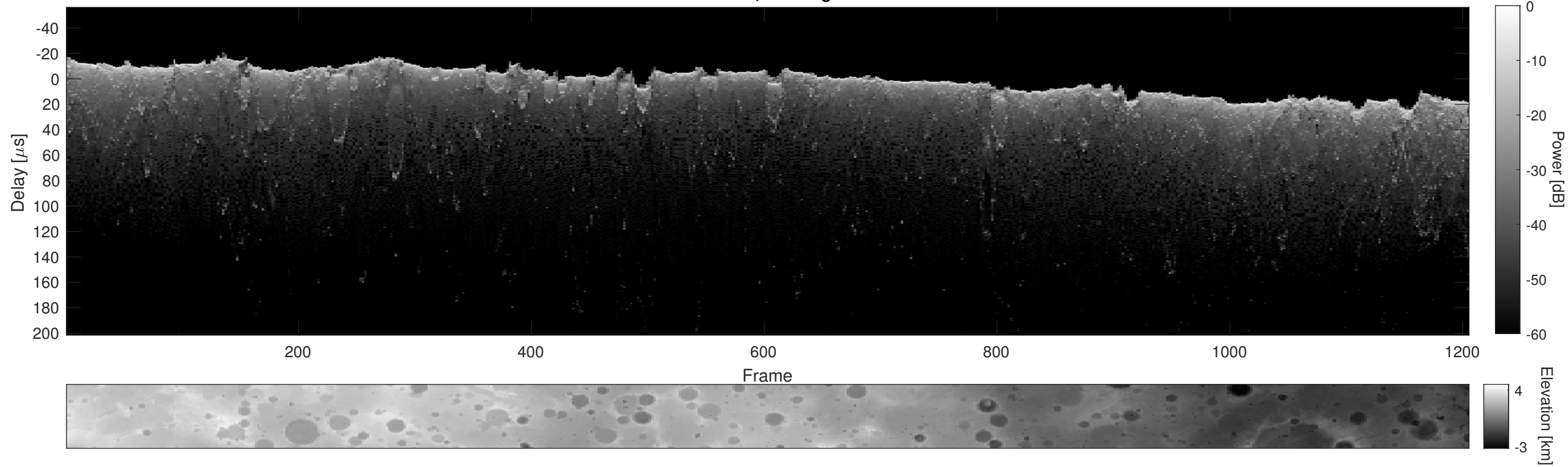
Orbit 6222, Cluttergram
