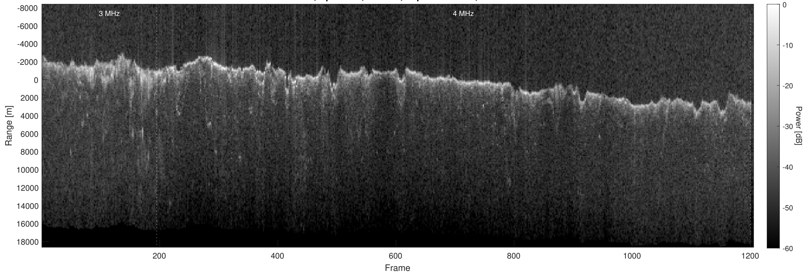
Orbit 6222, Optimized, Window, Depth-Corrected, Channel 2
