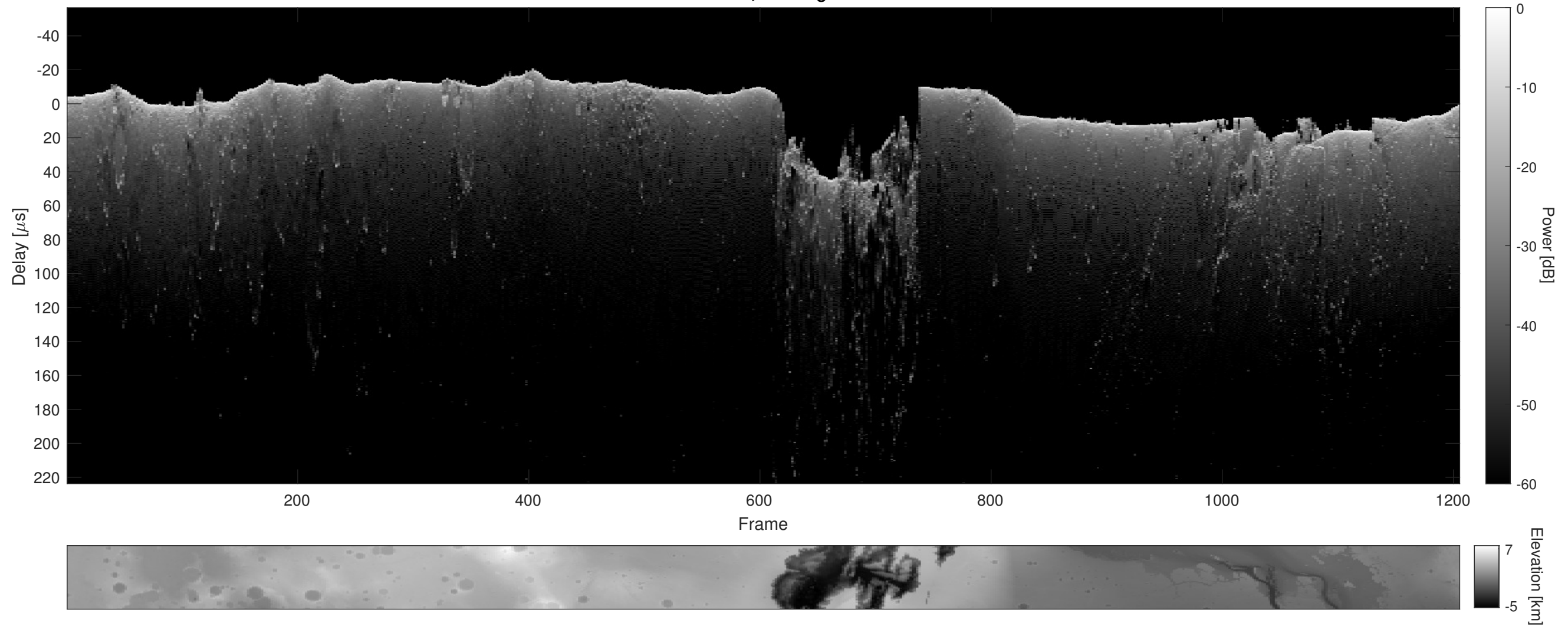
Orbit 6223, Cluttergram
