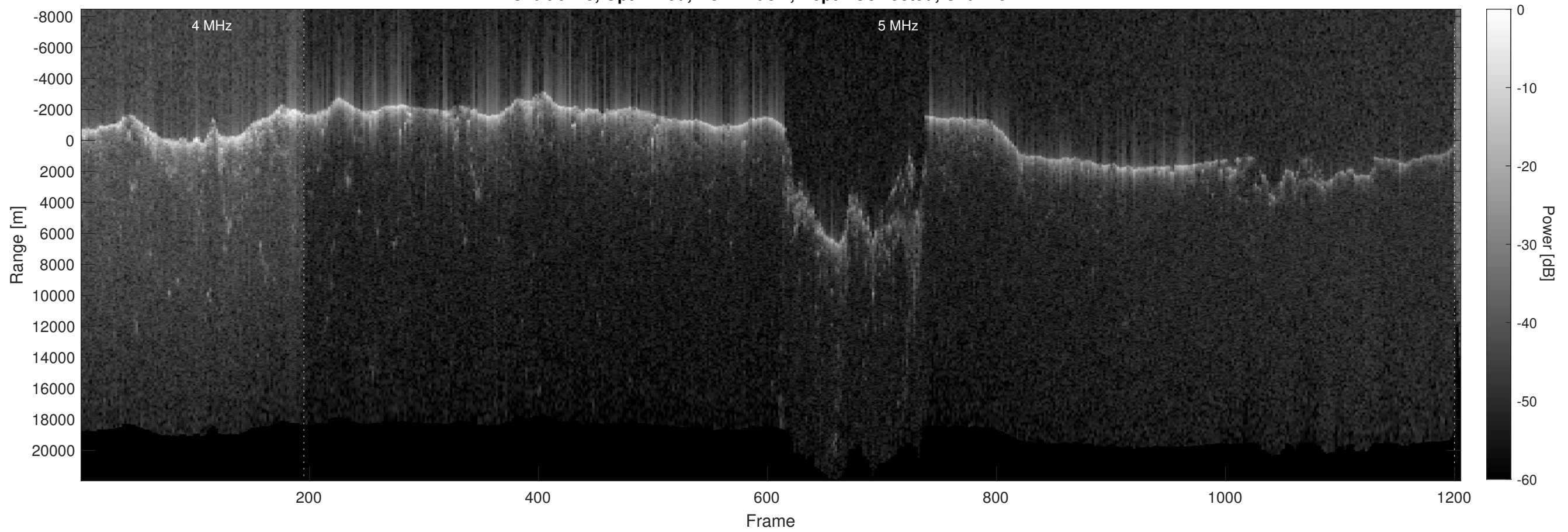
Orbit 6223, Optimized, No Window, Depth-Corrected, Channel 2
