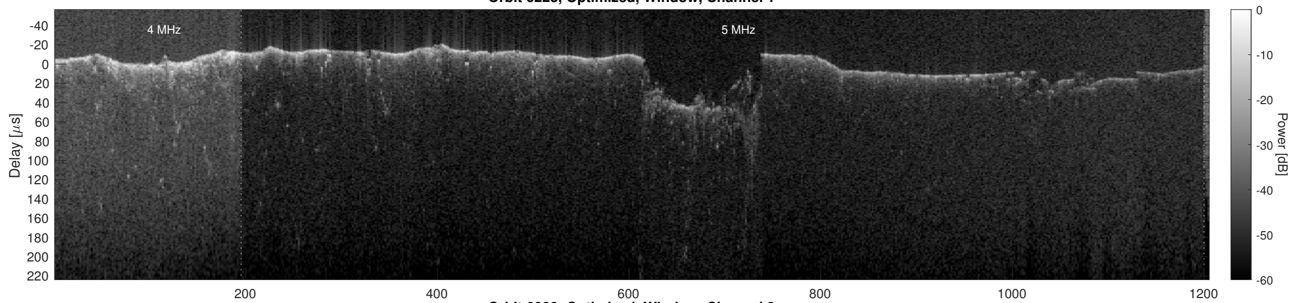
Orbit 6223, Optimized, Window, Channel 2
